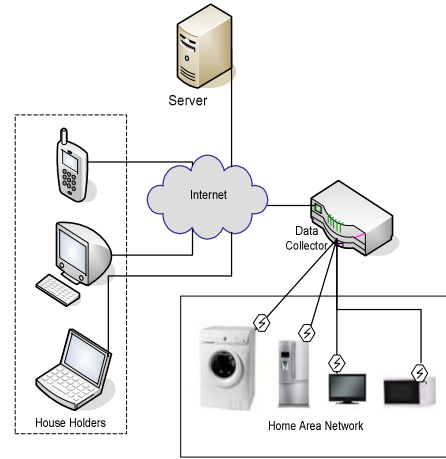
Figure 1: DEHEMS System Architecture
