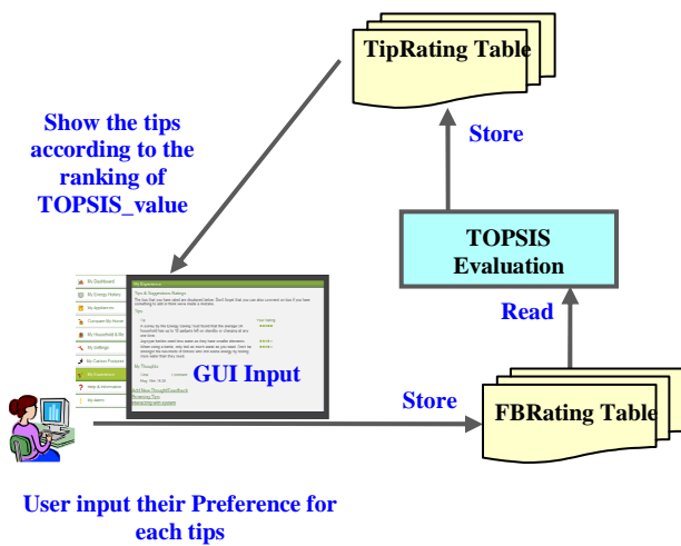
Figure 3: TOPSIS Architecture
