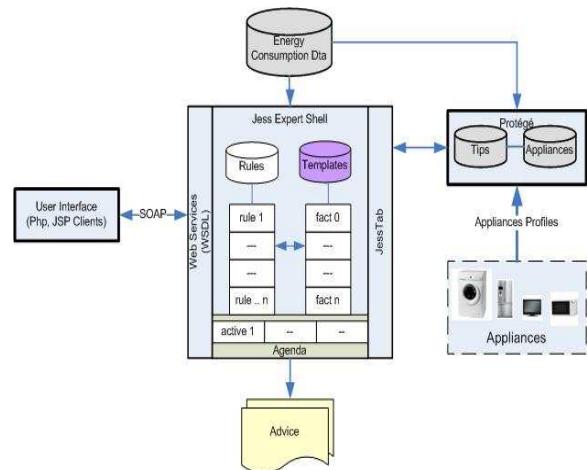
Figure 2: System Architecture
