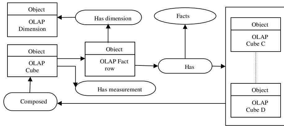
Figure 3. Composite OLAP
